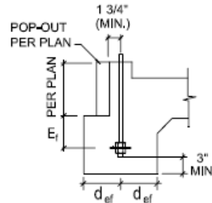
CURB SECTION
