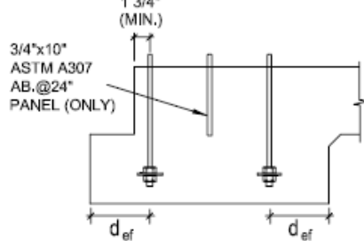
EXTERIOR SLAB ELEVATION
