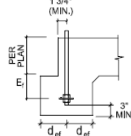
EXTERIOR SLAB SECTION
