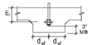
INTERIOR SLAB SECTION
